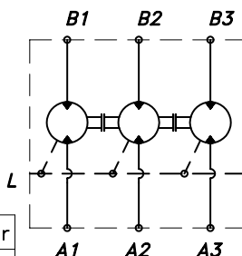
HYDRAULIC SCHEME
